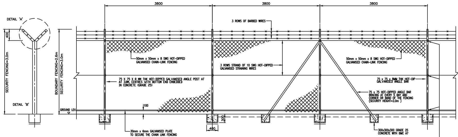
TYPICAL ELEVATION OF FENCING
