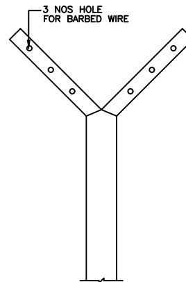
DETAIL 'A'
